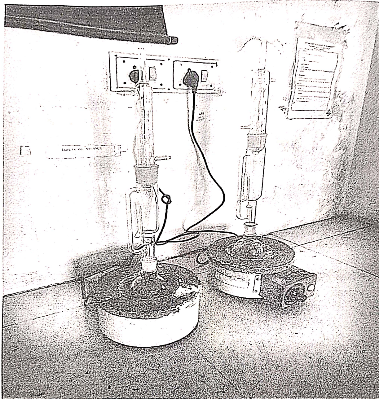
Soxlet Apparatus
